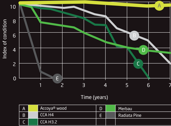
Figure 2: DECAY RATES OF FUNGUS CELLAR STAKELETS
