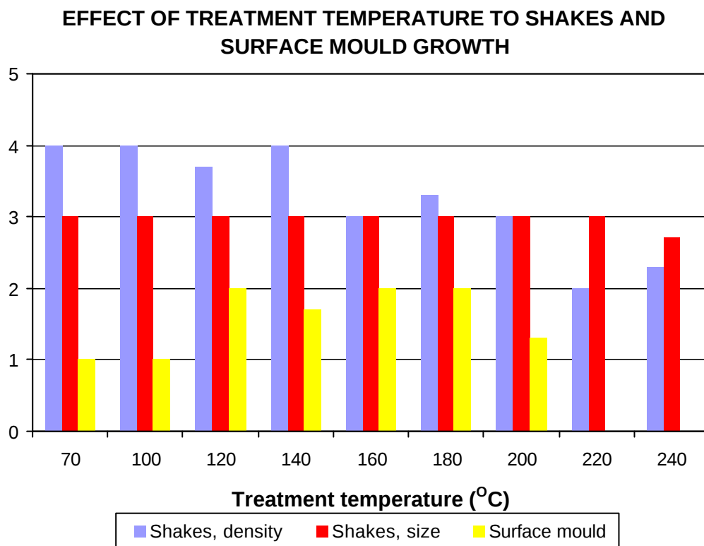
Figure 17-4. Effect of heat treatment temperature on surface shakes and fungal growth of pine panels. Heat treatment time of 3 hours. Outdoor exposure time of 6 months (source: VTT).
