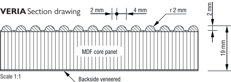
Example sketch using panels with 19 mm thickness
