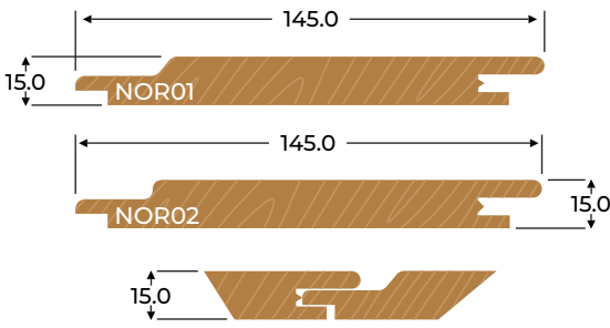
NOR01 & NOR02 ACCOYA ONLY AND SUITABLE FOR COATING
