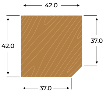
NWA4 ALSO AVAILABLE WITH ROUNDED CORNERS FOR COATED CLADDING
